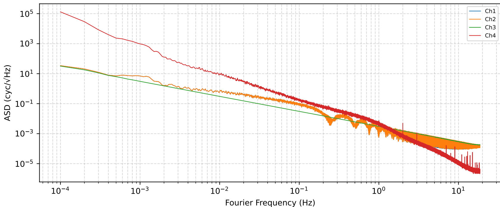
ASD:Delayline_11MHz_mix_UNDEL_DDS_400mVpp_ADC_on_inputs_1_2_and4_20260419_222428
